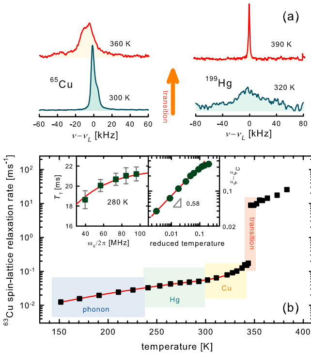
FIG. 1 (color online). (a) NMR lines of copper and mercury, below and above T_c . Frequency is relative to Larmor frequencies, 145.6 MHz for ^{65}\text{Cu} and 91.2 MHz for ^{199}\text{Hg} . Pulse excitation width is \sim 150 kHz. Copper lines are normalized to have the same integrals, while the low-temperature mercury line is multiplied by 10 after normalization. Significant motional narrowing is observed for mercury above T_c . (b) Spin-lattice relaxation measurements for ^{63}\text{Cu} . Left inset is frequency dependence at 280 K. Lines are fits obtained from a superposition of phonon and two defect diffusion processes (mercury and copper). Temperature ranges where each of the processes comes into play are indicated. Right inset is order parameter in dependence on reduced temperature.
