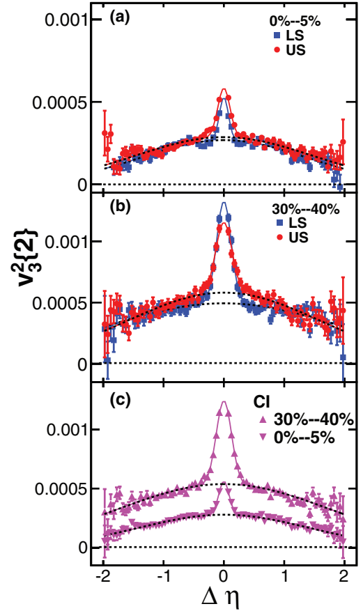
FIG. 2. (Color online) v_3^2\{2\} vs. the pseudorapidity separation of the particles in pairs for charged hadrons with 0.15 < p_T < 2.0 GeV/c within two centrality intervals in 200 GeV Au + Au collisions. Data are fit with narrow and wide Gaussians. Like sign (LS), unlike sign (US), and charge independent (CI) cases are shown with only statistical errors. The dashed curves under the peaks are the wide Gaussian fits.
