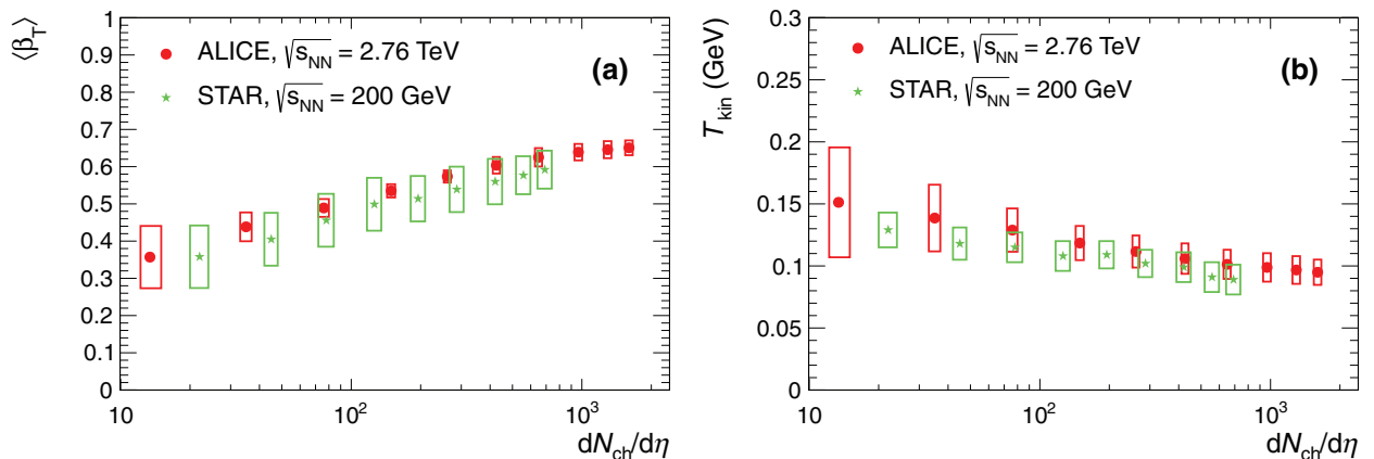
FIG. 11. (Color online) Blast-wave parameters (a) \langle\beta_T\rangle and (b) T_{\text{kin}} as a function of dN_{\text{ch}}/d\eta compared to previous results at \sqrt{s_{NN}} = 200 \text{ GeV} [5] (full systematic uncertainties for both experiments).
