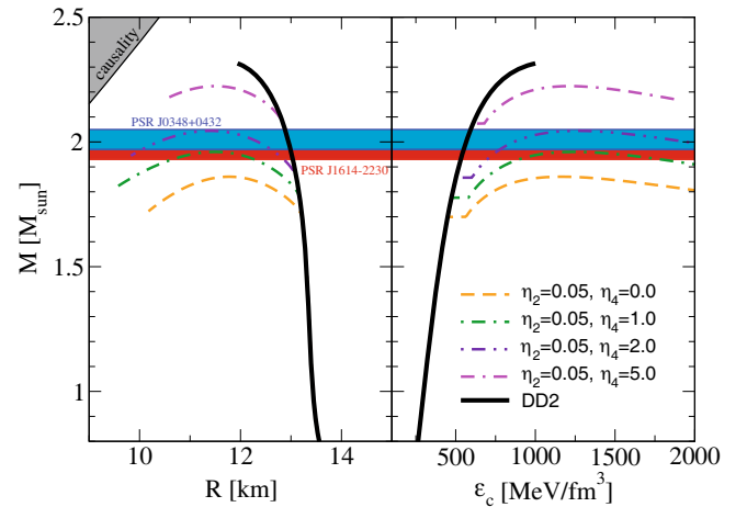
Fig. 2. (Color online) Left panel shows the M-R and the right panel the M-\epsilon_c diagram of compact star solutions within the model. We fix \eta_2 = 0.05 . The detachment from the hadronic branch given by the thick, black curve and the maximum mass depends on \eta_4 . Hybrid star branches appear in the same line styles as the corresponding EoS in fig. 1. Hatched regions mark experimental constraints from two heaviest sources, lower, red is [1], while higher, blue is [2].
