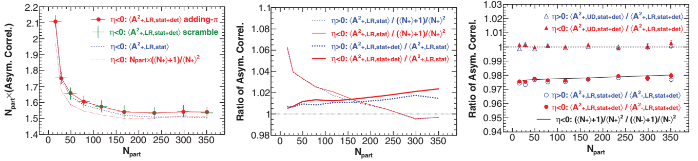
FIG. 19. (Color online) Left panel: Statistical fluctuation and detector effects in the charge asymmetry variance (multiplied by the number of participants N_{\text{part}} ) from the \eta < 0 region. The dotted curve shows the 1/N approximation using Eq. (B1), the dashed curve shows the statistical fluctuations \langle A_{-,\text{LR},\text{stat}}^2 \rangle obtained by use of the “50-50” method (see the text). The solid curve connecting the solid points shows the net effect of the statistical fluctuations and detector non-uniformities, \langle A_{-,\text{LR},\text{stat+det}}^2 \rangle , obtained by the adding- \pi method, and the crosses shows the same but obtained from the “scramble” method. See the text for details. Middle panel: The statistical fluctuation effects relative to the 1/N approximation (thin curves) and the effects due to the imperfect detector (thick curves). The dashed curves are for the region \eta > 0 and the solid curves are for \eta < 0 . Right panel: The ratios of the statistical fluctuation and detector effects \langle A_{+,\text{LR},\text{stat+det}}^2 \rangle / \langle A_{-,\text{LR},\text{stat+det}}^2 \rangle and \langle A_{+,\text{UD},\text{stat+det}}^2 \rangle / \langle A_{-,\text{LR},\text{stat+det}}^2 \rangle , separately for the \eta > 0 and \eta < 0 regions. The \phi -acceptance correction was applied for the results in this figure. The error bars are statistical only.
