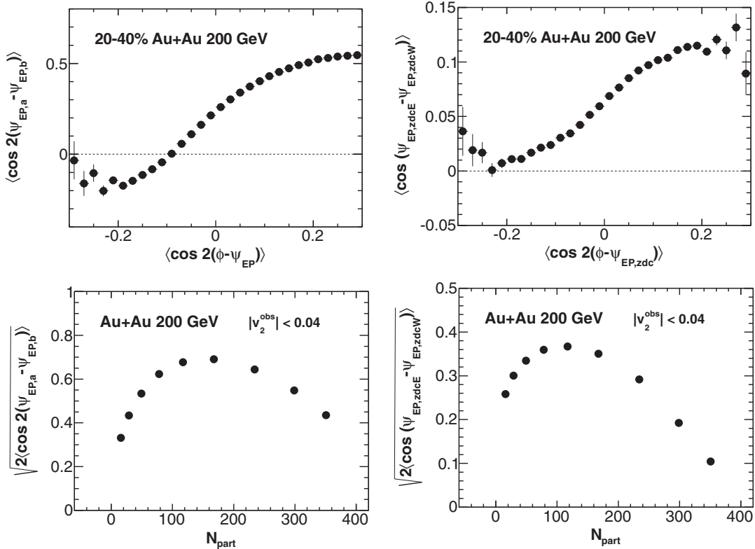
FIG. 25. The TPC second-harmonic (upper left) and ZDC-SMD first harmonic (upper right) event-plane resolution as a function of v_2^{\text{obs}} in 20–40% central Au + Au collisions. The TPC second-harmonic (lower left) and ZDC-SMD first harmonic (lower right) event-plane resolution for events with |v_2^{\text{obs}}| < 0.04 as a function of centrality. The error bars are statistical only.
