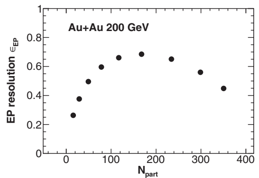
FIG. 23. The second-harmonic event-plane resolution of subevents ( \eta < 0 and \eta > 0 ) as a function of the number of participants. The statistical errors are smaller than the symbol sizes.
