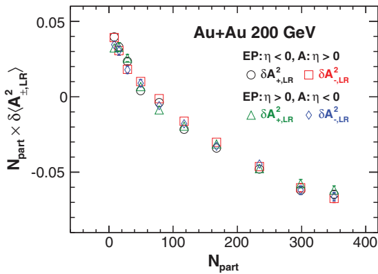
FIG. 22. (Color online) Dynamical charge asymmetry variance after removing the statistical and detector effects, \delta\langle A^2_{\pm,LR} \rangle = \langle A^2_{\pm,LR} \rangle - \langle A^2_{\pm,LR,stat+det} \rangle , scaled by the number of participants N_{\text{part}} . The results are consistent between positive and negative \eta regions and between positive and negative charges. Error bars are statistical only.
