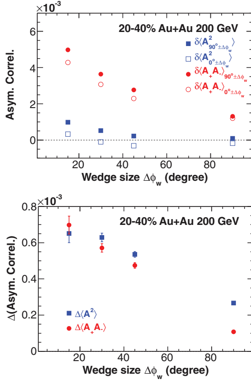
FIG. 8. (Color online) The wedge size dependencies of charge multiplicity asymmetry correlations (upper panel), and their differences between out of plane and in plane, \Delta\langle A^2_{\Delta\phi_w} \rangle and \Delta\langle A_+ A_- \rangle_{\Delta\phi_w} (lower panel), for 20–40% central Au + Au collisions. The error bars are statistical only.
