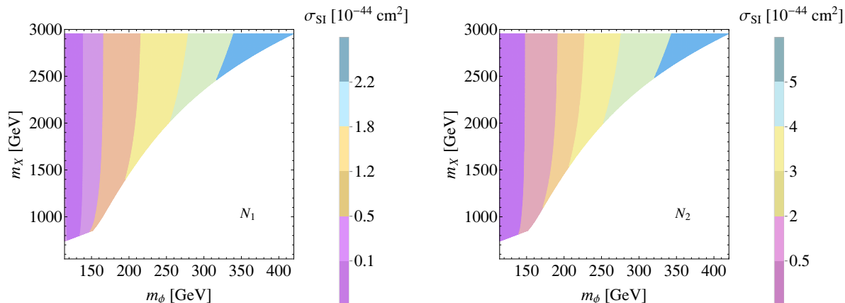
Figure 7. Left (right) panel: Majorana dark matter N_1 ( N_2 ) direct detection cross section in the m_\phi - m_X plane for m_{N_2} = 1.5m_{N_1} . We impose the LHC bound on \sin\theta and the LUX experiment constraints.
