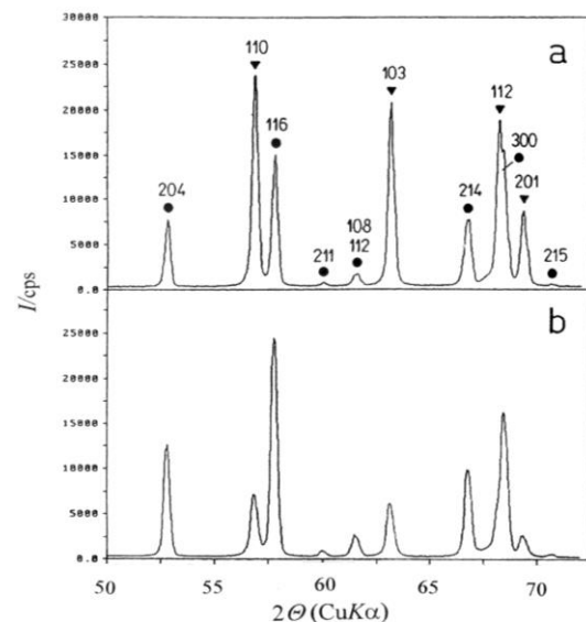
Fig. 1. X-ray diffraction patterns of the system ZnO ( A = 0.5 , ▼) + \alpha - \text{Al}_2\text{O}_3 ( B = 0.5 , ●): (a) original sample, (b) the sample doped with B_a = 0.667 . Radiation \text{CuK}\alpha . [12]
