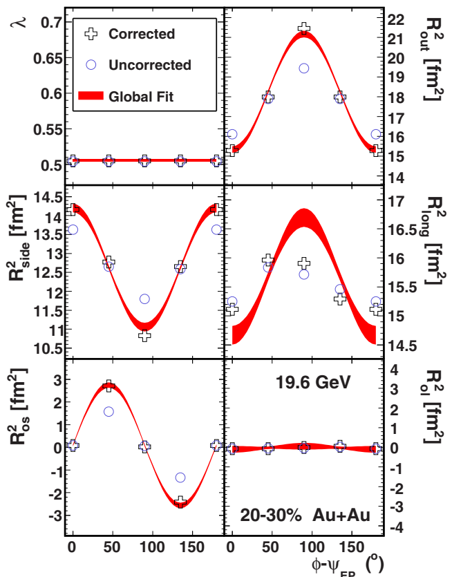
FIG. 4. (Color online) Examples of the angular oscillations of the HBT radii relative to the event plane from 20%–30% central, 19.6-GeV Au + Au collisions for 0.15 < k_T < 0.6 GeV/ c . Open circles show the radii before correction for finite-bin-width and event-plane resolution. Open cross symbols demonstrate that correcting these effects increases the oscillation amplitude. The corrected and uncorrected results are obtained with the HHLW fit method (see text) before and after the correction algorithm (Sec. VB) is applied. The points at 0^\circ are repeated on the plot at 180^\circ for clarity. The solid bands show the Fourier decomposition directly extracted using a global fit (Sec. VC) to all four angular bins; the width of the bands represent 1\sigma uncertainties from the fit. The value of \lambda is consistent for the two methods.
