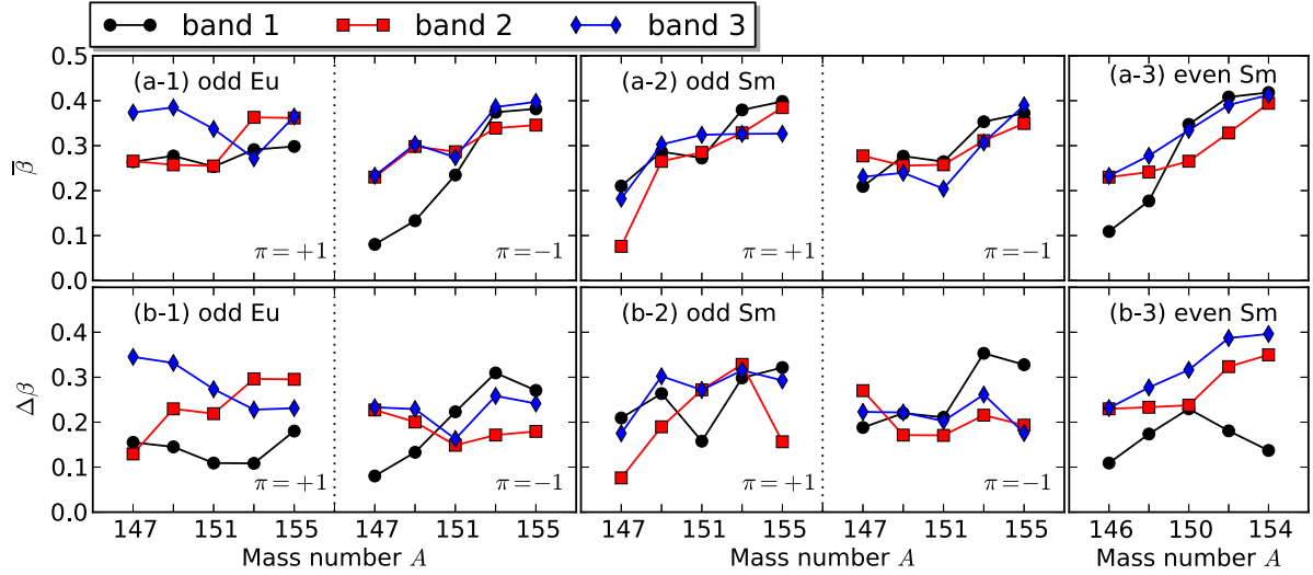
FIG. 8. Evolution of characteristic mean-field quantities calculated for the lowest three positive- ( \pi = +1 ) and negative-parity ( \pi = -1 ) bands of the odd- A Eu and Sm nuclei, and K^\pi = 0^+ bands in the even- A Sm isotopes, as functions of mass number: the mean value \bar{\beta} (a) and variance \Delta\beta (b) of the equilibrium deformation parameter for the bandhead state. “band 1,” “band 2,” and “band 3” denote the lowest, second-lowest, and third-lowest bands, respectively. See the main text for the definition of each quantity.
