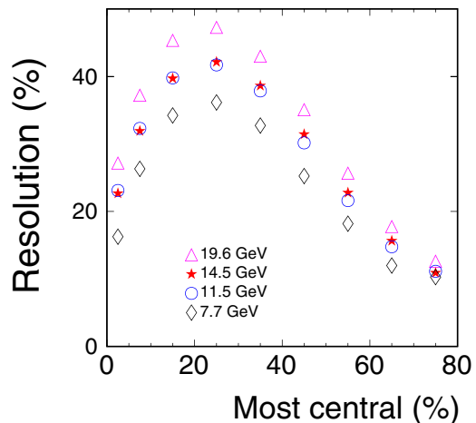
FIG. 2. The subevent plane resolution for several beam energies versus centrality with 5% being the most central.
