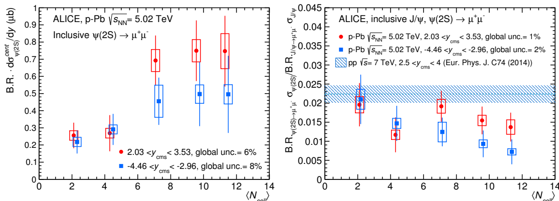
Figure 2. Left: \psi(2S) production cross sections shown as a function of \langle N_{\text{coll}} \rangle for both p-Pb and Pb-p collisions. Right: \text{B.R.}_{\psi(2S) \rightarrow \mu^+ \mu^-} \sigma_{\psi(2S)} / \text{B.R.}_{J/\psi \rightarrow \mu^+ \mu^-} \sigma_{J/\psi} shown as a function of \langle N_{\text{coll}} \rangle and compared to the pp value (line), with a band representing its uncertainty. In both figures, vertical error bars correspond to statistical uncertainties, while the open boxes represent the systematic uncertainties. The Pb-p points are slightly shifted in \langle N_{\text{coll}} \rangle to improve visibility.
