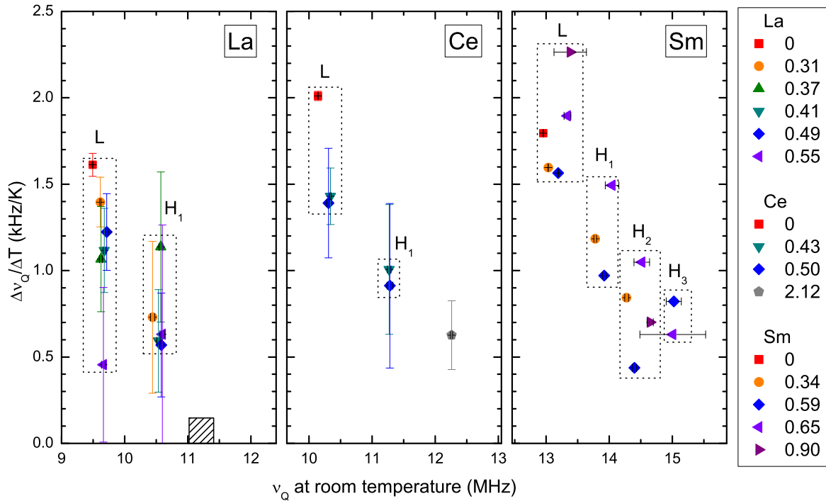
FIG. 5. Temperature sensitivity of the quadrupolar frequency, as a function of the peak position at room temperature. \Delta v_Q/\Delta T is calculated from measurements at room temperature and at T = 150\text{--}160 K. The legend indicates x_{\text{NQR}}/x_{\text{FSWT}} . For x_{\text{NQR}} < x_{\text{FSWT}} , each dotted box groups the points belonging to the same frequency branch (L, H_1 , H_2 , H_3 ) as defined in Fig. 3. For La-based samples, the hatched rectangle about \nu_Q \approx 11.2 MHz indicates the frequency range over which \Delta v_Q/\Delta T goes from weak ( x_{\text{NQR}}/x_{\text{FSWT}} = 1.19 ) to zero or negative ( x_{\text{NQR}}/x_{\text{FSWT}} = 1.90 ). Error bars for the Sm-based samples are not shown, as they exceed the actual point dispersion for each frequency branch, suggesting overestimation due to more complex spectra.
