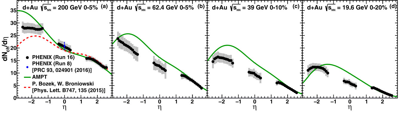
FIG. 12. The dN_{\text{ch}}/d\eta vs. \eta in central d + \text{Au} collisions at \sqrt{s_{\text{NN}}} = (a) 200, (b) 62.4, (c) 39, and (d) 19.6 GeV. The solid [green] curves are the AMPT calculations in similar centrality bins. The dashed [red] curve in panel (a) is a hydrodynamic prediction from Ref. [40] for 0%–5% central d + \text{Au} collisions at \sqrt{s_{\text{NN}}} = 200 GeV.
