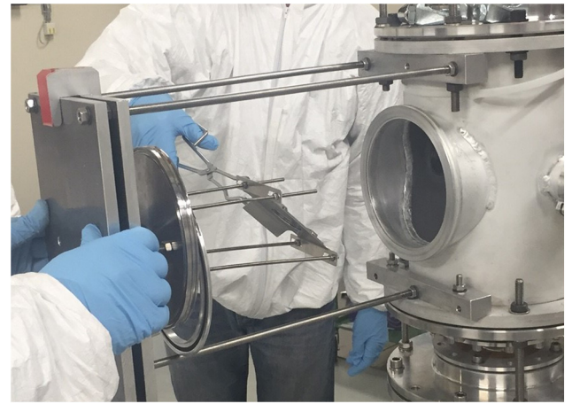
Fig. 5. Insertion of the ^7\text{Be} radioactive target in the setup, with a support independent of the telescope detector installed from the opposite side of the chamber.
