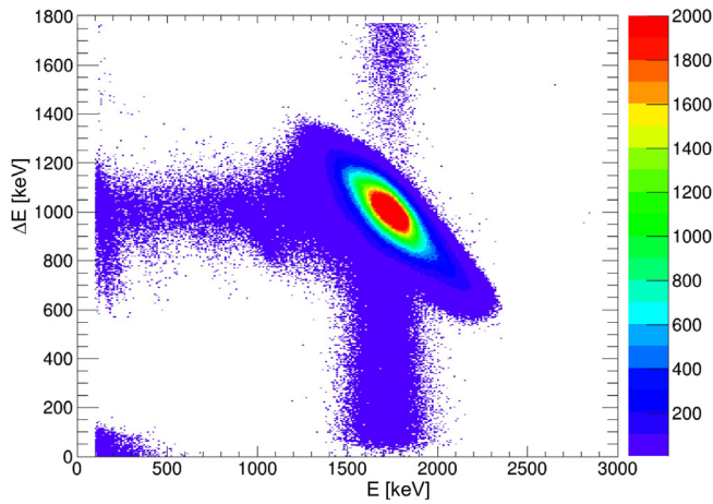
Fig. 8. \Delta E - E scatter plot measured from the {}^6\text{Li}(n,\alpha) reaction, with the tritons locus clearly visible. The wide energy spread was due to the emission depth and angle in the target, and to the wide range of incidence angles on the detector.
