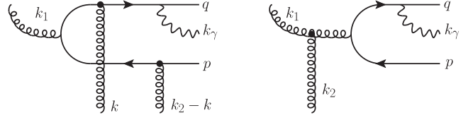
FIG. 2. Examples for NLO diagrams for photon production in the high-energy limit. In the left diagram the gluon from the proton emits a q\bar{q} pair which then scatters on the dense nucleus. In the right diagram the gluon scatters on the nucleus and then produces a q\bar{q} pair and a photon. The complete NLO contribution includes diagrams where the photon is emitted from the antiquark line, or from a virtual quark-antiquark state (not shown) in the case of single-inclusive photon production.
