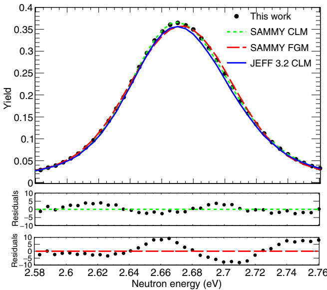
FIG. 8. SAMMY fits and residuals of the largest ^{242}\text{Pu} capture resonance using free gas (FGM) and a crystal lattice (CLM) models to describe the Doppler broadening. The fit obtained using the resonance parameters in JEFF-3.2 or ENDF/B-VII.1 (CLM) is shown as a reference.
