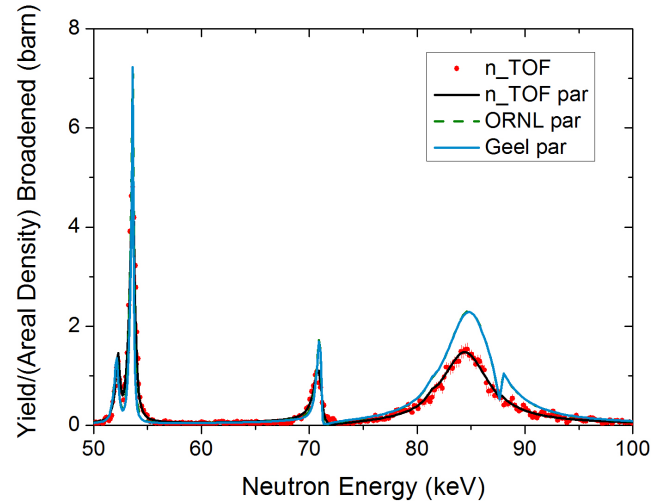
FIG. 7. R -matrix analysis from 50 to 100 keV. The n _TOF data (red points) are compared with the description of ORNL [5] (dashed green line), Geel [6] (blue line), and the present work (black line). Geel and ORNL are coincident from 60 to 100 keV.
