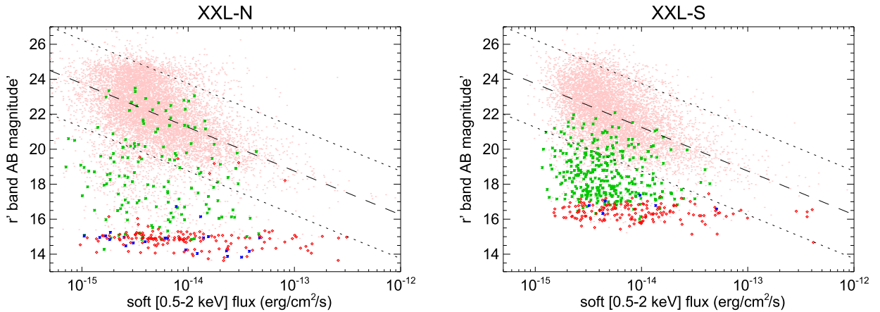
Fig. 7. Optical vs. X-ray flux for XXL-N (left) and XXL-S (right). The r' magnitude of the primary counterpart is plotted against the broad-band soft flux [0.5–2 keV]. Symbols and colour-codes are as follows: pink dots correspond to magnitudes available only from either CFHT (preferred) or SDSS (in XXL-N), or either BCS (preferred) or DECam (in XXL-S); green asterisks to stars identified as such by their spectroscopic redshift (star flag 1); red diamonds to stars identified visually (star flag 2); blue asterisks to spectroscopic and visual stars (star flag 3). The dashed and dotted lines mark the AGN locus of X/O = 0 \pm 1 (e.g. Brandt & Hasinger 2005).
