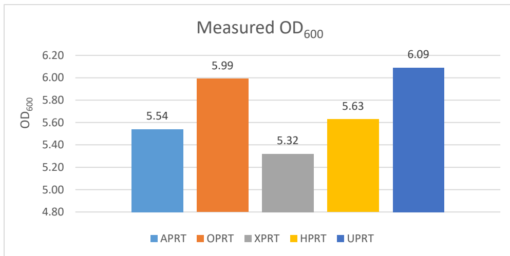
Figure 3.9. Measured values of 100 μL of over-night cultures mixed with 900 μL of LB medium.
