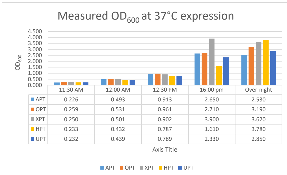
Figure 3.9. Measured values of 100 μL of over-night cultures mixed with 900 μL of LB medium.
