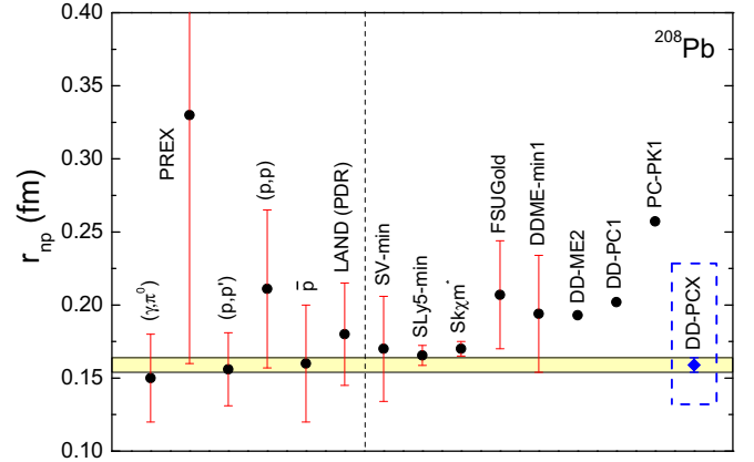
FIG. 3. The neutron skin thickness for 208 Pb predicted by different experiments and nuclear energy density functionals. The experimental data are taken from (\gamma, \pi^0) [48], PREX [16], (p, p) [19], (p, p) [49], \bar{p} [50], LAND(PDR) [51]. The calculations with the nonrelativistic interactions: SV-min [4], SLy5-min [31], Sk \chi m* [47], and relativistic interactions: FSUGold [46], DDME-min [31], DD-ME2 [8], DD-PC1 [7], PC-PK1 [9].
