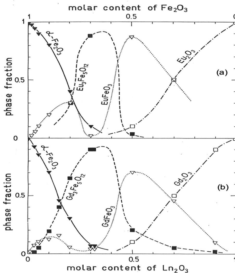
Figure 6. Approximate molar fractions (at RT) of the crystalline phases in the systems \alpha\text{-Fe}_2\text{O}_3\text{-Ln}_2\text{O}_3 , Ln = Eu (a), Gd (b), as a function of the initial molar fractions of \alpha\text{-Fe}_2\text{O}_3 and \text{Ln}_2\text{O}_3 . Samples were prepared at 1170 K [23].
