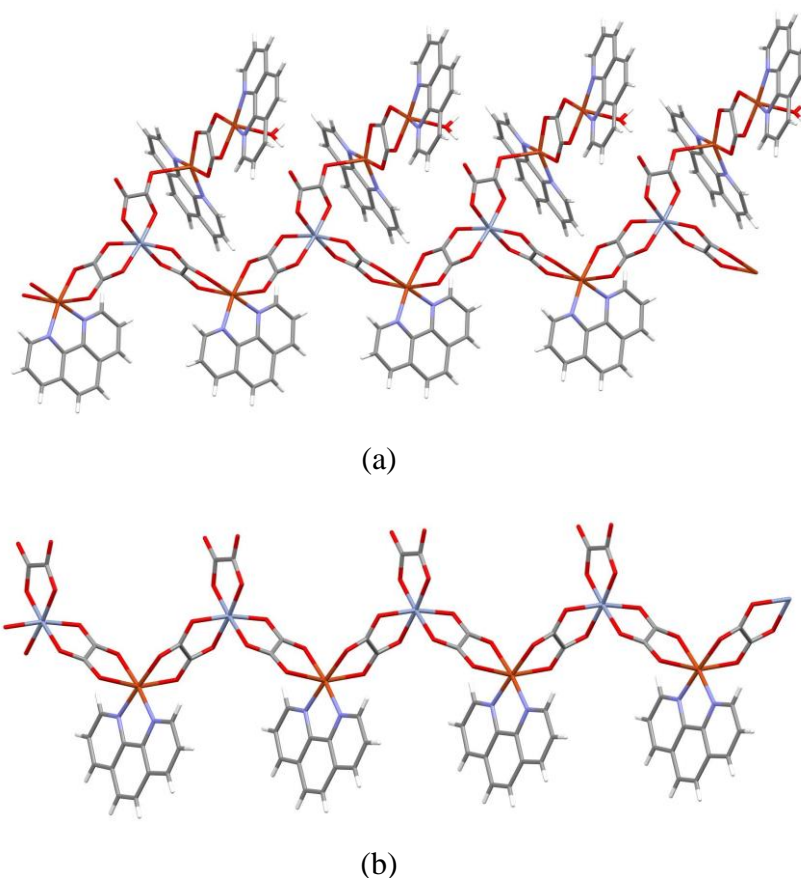
Slika 74. Kristalna struktura spoja \{[\text{CrCu}_3(\text{phen})_3(\text{H}_2\text{O})(\text{C}_2\text{O}_4)_4][\text{Cu}(\text{phen})\text{Cr}(\text{C}_2\text{O}_4)_3] \cdot 2\text{CH}_3\text{CN} \cdot 3\text{H}_2\text{O}\}_n ( 9o ): (a) kationski i (b) anionski lanac
