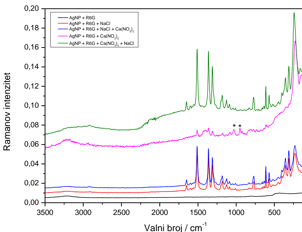
Slika 15. SERS spektri R6G ( 5 \times 10^{-6}\text{ mol dm}^{-3} ) u svježe pripravljenom koloidu srebra: bez agregirajućeg sredstava (crno), s NaCl ( c = 1 \times 10^{-2}\text{ mol dm}^{-3} ) (crveno), s NaCl ( c = 1 \times 10^{-2}\text{ mol dm}^{-3} ) i \text{Ca}(\text{NO}_3)_2 ( c = 1 \times 10^{-3}\text{ mol dm}^{-3} ) (plavo), s \text{Ca}(\text{NO}_3)_2 ( c = 1 \times 10^{-3}\text{ mol dm}^{-3} ) (ružičasto), s \text{Ca}(\text{NO}_3)_2 ( c = 1 \times 10^{-3}\text{ mol dm}^{-3} ) i NaCl ( c = 1 \times 10^{-2}\text{ mol dm}^{-3} ) (zeleno).
