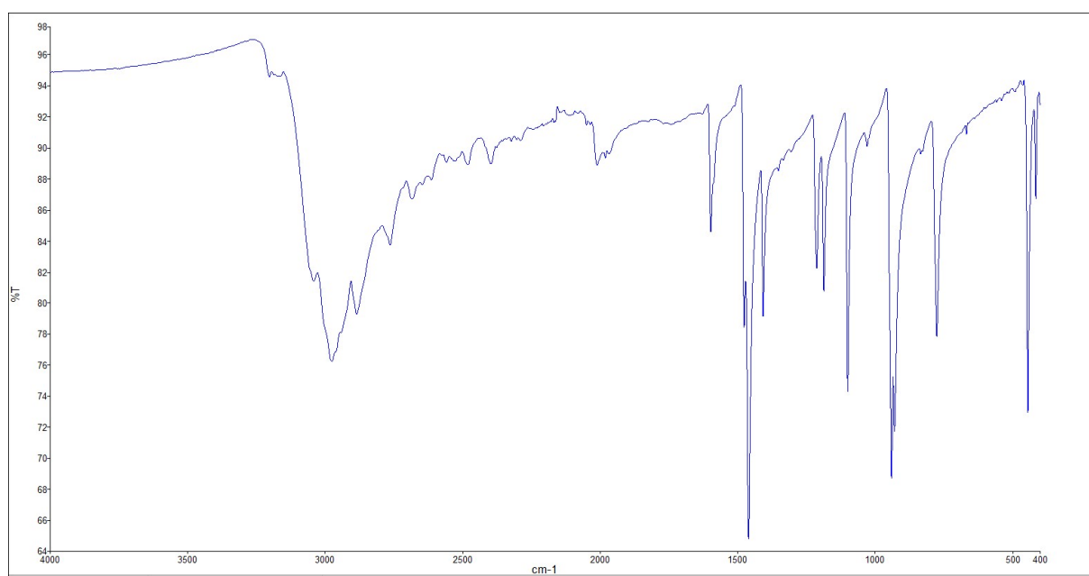
Slika D4. IR spektar bromidne soli propan-1,3-diamina, \text{H}_2(1,3\text{-DAP})\text{Br}_2
