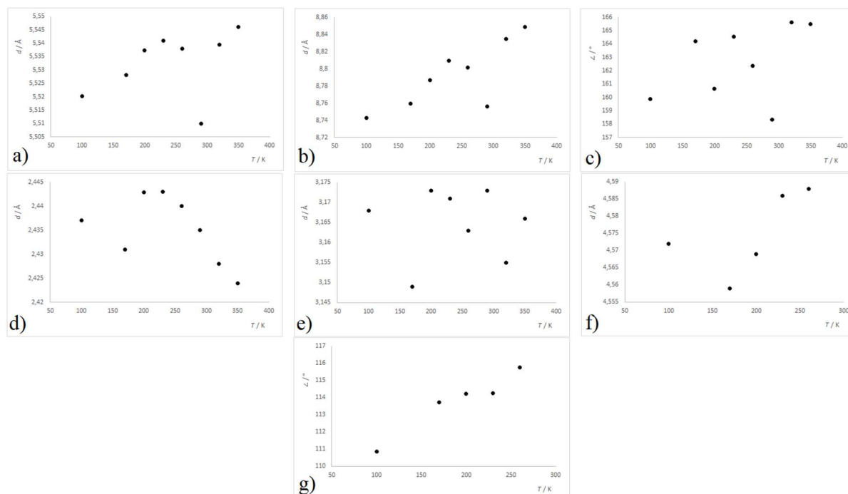
Slika 32. Grafički prikazi d(\text{Cu—Cu})_{\text{ip}} (a), d(\text{Cu—Cu})_{\text{oop}} (b), \angle(\text{Cu—Br}_{\text{kv}}\text{—Cu}) (c), d(\text{Cu—Br}_{\text{kv}})_{\text{s}} (d), d(\text{Cu—Br}_{\text{kv}})_{\text{l}} (e), d(\text{N—N}) (f), \angle(3\text{C atoma}) (g) u ovisnosti o temperaturi za spoj \text{H}_2(1,3\text{-DAP})[\text{CuBr}_4]
