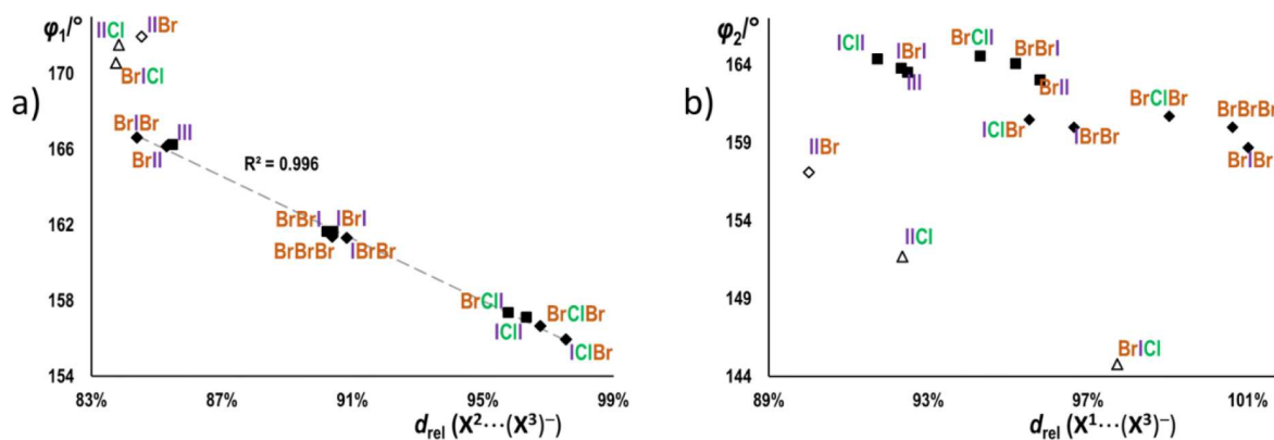
Figure 4. Correlation between the relative halogen bond length ( d_{\text{rel}} = d(\text{X} \cdots (\text{X}^3)^-)/[r_{\text{vdW}}(\text{X}) + r_{\text{p}}((\text{X}^3)^-)] and the halogen bond angle ( \phi ) for the (a) halogen bond with the donor atom on the pyridine ring ( \text{C}2-\text{X}^2 \cdots (\text{X}^3)^- ) and (b) on the benzyl ring ( \text{C}2-\text{X}^1 \cdots (\text{X}^3)^- ). Type I structures are represented by black circles, and type II structures are represented with white circles with a black border.
