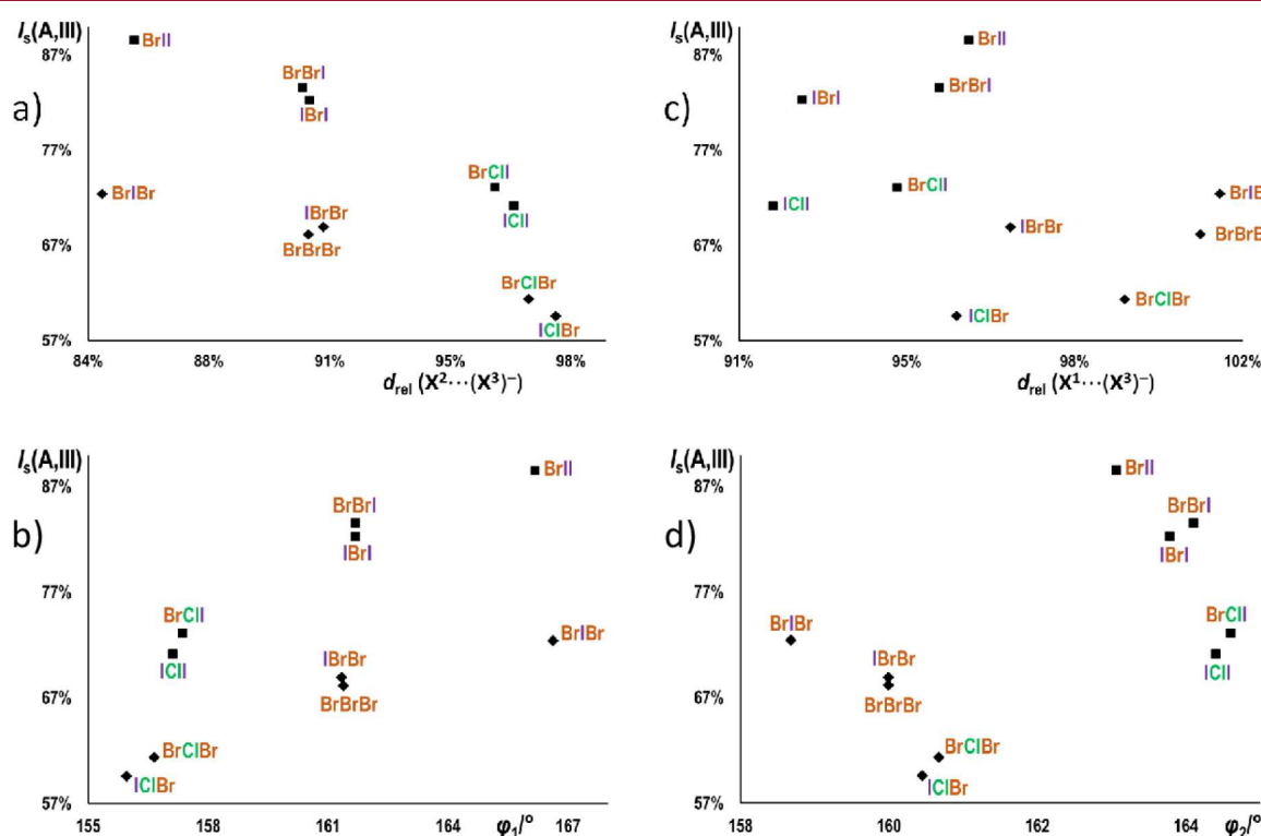
Figure 5. Correlations between the halogen bond parameters and the isostructurality index with respect to III ( I_s(\text{A}, \text{III}) , \text{A} \neq \text{III} ) for structures of the type I series with (a) relative length of the \text{X}^2 \cdots \text{X}^3 halogen bond, d_{\text{rel}}(\text{X}^2 \cdots \text{X}^3) plot; (b) angle of the \text{X}^2 \cdots \text{X}^3 halogen bond, \phi_1 plot; (c) relative length of the \text{X}^1 \cdots \text{X}^3 halogen bond, d_{\text{rel}}(\text{X}^1 \cdots \text{X}^3) , (d) angle of the \text{X}^1 \cdots \text{X}^3 halogen bond, \phi_2 . Structures of iodide salts are represented by squares and bromide salts as rhombi.
