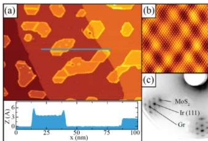
Figure 19. MBE growth of \text{MoS}_2/\text{Gr} heterostructure. (a) STM topograph after growth of \text{MoS}_2 islands with the on \text{Gr}/\text{Ir}(111) . The height profile along the indicated blue line is shown below. (b) Atomically resolved topograph of a \text{MoS}_2 island. (c) Section of a corresponding 80 eV LEED pattern. The first-order reflections of \text{MoS}_2 , \text{Ir}(111) and \text{Gr} are indicated. [Adopted from Ref. 58 ].
