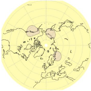
Appendix Figure C3 Signal variance (sig var) of geopotential heights at 200 hPa [ m^2 ] in the 57 non-ENSO years in January (left), February (middle), and March (right) in the ICTP AGCM experiments: Ctrl, TroAtl, TroInd, TroPac, Tropics, and Clim, respectively. The non-ENSO years were selected from 156 years (1855-2010) according to the strength of the Niño3.4 index in the JFM season.
