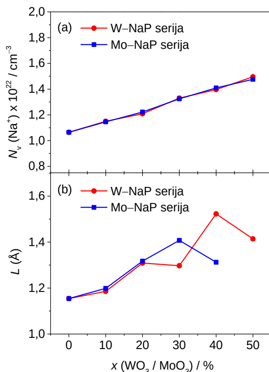
Slika 73. (a) Gustoća broja natrijevih iona, N_v(\text{Na}^+) i (b) Sidebottomova duljina, L , u ovisnosti o udjelu \text{WO}_3 i \text{MoO}_3 iz serija stakala x\text{WO}_3-40\text{Na}_2\text{O}-(60-x)\text{P}_2\text{O}_5 i x\text{MoO}_3-40\text{Na}_2\text{O}-(60-x)\text{P}_2\text{O}_5 , x = 0-50 \% .
