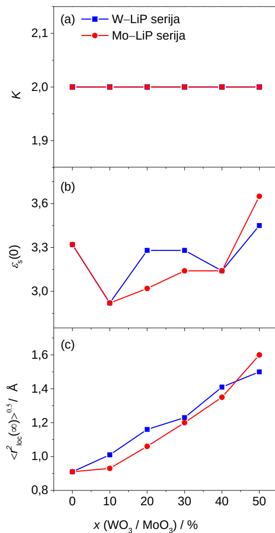
Slika 58. Trendovi ovisnosti (a) parametra K , (b) plateau-a skalirane permitivnosti, \epsilon_s(0) , i (c) prostornog dosega lokaliziranih skokova iona natrija, \langle r_{loc}^2(\infty) \rangle^{0.5} , o udjelu \text{WO}_3 i \text{MoO}_3 u serijama stakala x\text{WO}_3\text{--}40\text{Li}_2\text{O--}(60-x)\text{P}_2\text{O}_5 i x\text{MoO}_3\text{--}40\text{Li}_2\text{O--}(60-x)\text{P}_2\text{O}_5 , x = 0\text{--}50\% .
