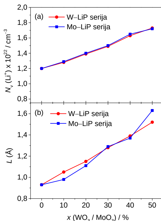
Slika 56. (a) Gustoća broja litijevih iona, N_v(\text{Li}^+) , i (b) Sidebottomova duljina, L , u ovisnosti o udjelu \text{WO}_3 i \text{MoO}_3 u serijama stakala x\text{WO}_3-40\text{Li}_2\text{O}-(60-x)\text{P}_2\text{O}_5 i x\text{MoO}_3-40\text{Li}_2\text{O}-(60-x)\text{P}_2\text{O}_5 , x = 0-50 %.
