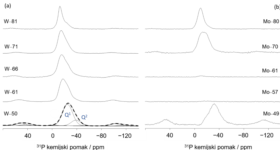
Slika 34. ^{31}\text{P} MAS-NMR spektri serija stakala (a) x\text{WO}_3-(100-x)\text{P}_2\text{O}_5 i (b) x\text{MoO}_3-(100-x)\text{P}_2\text{O}_5 , x = 49-81 %.
