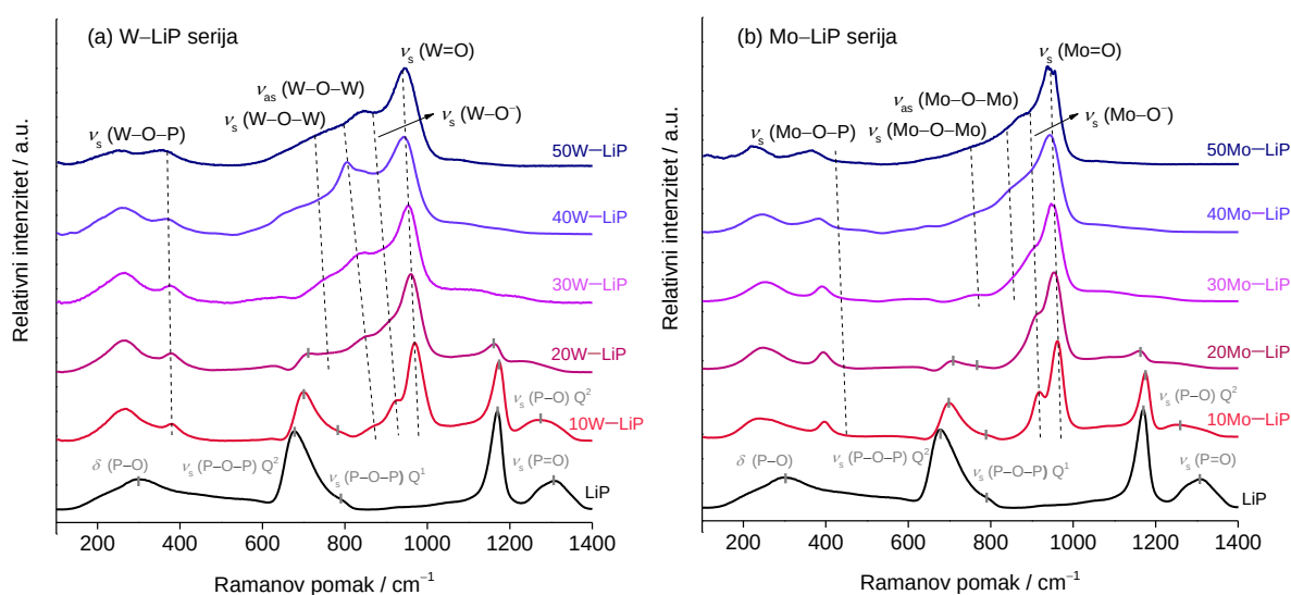
Slika 45. Ramanovi spektri serija stakala (a) xWO_3-40Li_2O-(60-x)P_2O_5 i (b) xMoO_3-40Li_2O-(60-x)P_2O_5 , x = 0-50 \% .
