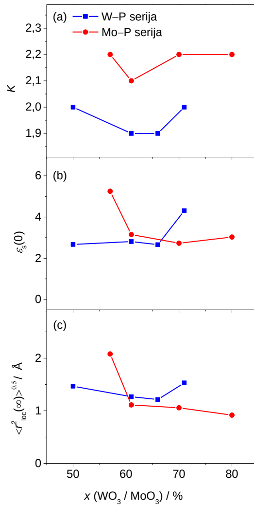
Slika 43. Trendovi ovisnosti (a) parametra K , (b) plateau-a skalirane permitivnosti, \epsilon_s(0) , i (c) prostornog dosega lokaliziranih skokova polarona, \langle r_{loc}^2(\infty) \rangle^{0.5} , o udjelu \text{WO}_3 i \text{MoO}_3 u serijama stakala x\text{WO}_3-(100-x)\text{P}_2\text{O}_5 i x\text{MoO}_3-(100-x)\text{P}_2\text{O}_5 , x = 50-80 \% .
