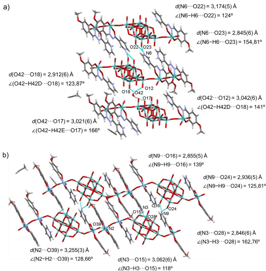
Slika 96. Prikaz vodikovih veza u spoju [\text{Mo}_2\text{O}_4(\text{H}_2\text{4OMeSalNH})(\text{H4OMeSalNH})][\text{MoO}_2(\text{H4OMeSalNH})\text{Mo}_8\text{O}_{26}] \cdot 2\text{MeCN} \cdot \text{H}_2\text{O} duž osi: a) a i b) b.
