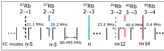
FIG. 2. Relative positions of comb lines within the FC spectrum with respect to the ^{85}\text{Rb} |5S_{1/2}; F = 3\rangle \rightarrow |5P_{3/2}; F' = 2, 3, 4\rangle and ^{87}\text{Rb} |5S_{1/2}; F = 2\rangle \rightarrow |5P_{3/2}; F' = 1, 2, 3\rangle hyperfine transitions for the FC parameters used in the experiment. Note that, when the n -th comb mode is resonant with the ^{87}\text{Rb} |5S_{1/2}; F = 2\rangle \rightarrow |5P_{3/2}; F' = 3\rangle transition, the (n + 14) -th comb mode is 0.4 MHz blue detuned from (i.e., almost in resonance with) the ^{85}\text{Rb} |5S_{1/2}; F = 3\rangle \rightarrow |5P_{3/2}; F' = 4\rangle transition.
