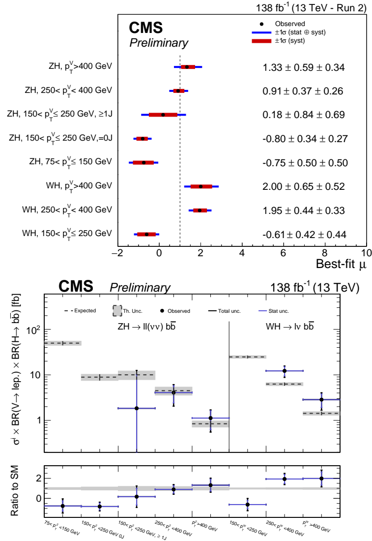
Figure 5.6: Measured STXS signal strengths from the fit (top). Measured values of \sigma \times \mathcal{B} in the same STXS bins as for the signal strengths, combining all years (bottom).
