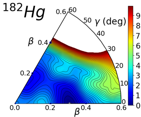
FIG. 6. Potential-energy surface (PES) for the nucleus ^{182}\text{Hg}_{102} , obtained by CDFT using the DDME2 functional used throughout the present work. All energies are normalized with respect to the binding energy of the corresponding ground state. The PES looks very similar to Fig. 18(a) of Ref. [83], produced for the same nucleus within the IBM-CM framework. See Sec. III for further discussion.
