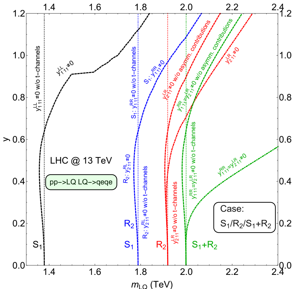
Figure 5. The leptptoquark parameter space limits for the S_1 , R_2 , and S_1+R_2 scenarios extracted from the pp \rightarrow LQ\bar{L}\bar{Q} \rightarrow jjee process search [1] performed at 13 TeV center-of-mass energy of proton-proton collisions at the LHC, using an integrated luminosity of 139 \text{ fb}^{-1} . See text for more details.
