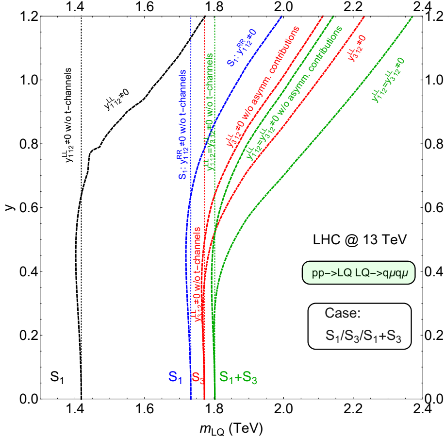
Figure 10. The leptoquark parameter space limits for the S_1 , S_3 , and S_1+S_3 scenarios extracted from the pp \rightarrow L\bar{Q}L\bar{Q} \rightarrow jj\mu\mu process search [1] performed at 13 TeV center-of-mass energy of proton-proton collisions at the LHC, using an integrated luminosity of 139 \text{ fb}^{-1} . See text for more details.
