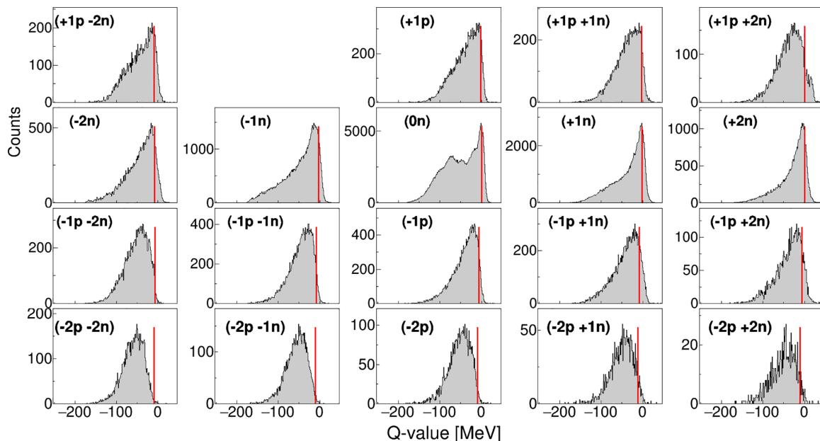
FIG. 6. Q -value distributions measured at \theta_{\text{lab}} = 35^\circ for the labeled transfer channels. The yield for the (+1p - 1n) channel could not be safely extracted due to partial overlap with the ^{118}\text{Sn} one. Vertical lines indicate the ground-to-ground state Q values.
