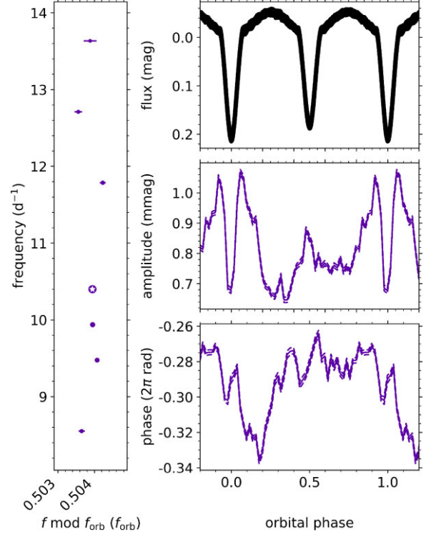
Figure C4. Tidally perturbed pulsation with frequency f = 10.399706(2)d^{-1} .
