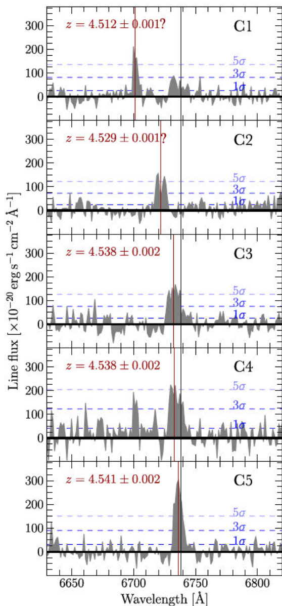
Figure 7. Optimally extracted 1D spectra of the five emitting sources in the vicinity of J1000+0234. The horizontal blue lines show the 1, 3, and 5\times rms noise level. The vertical red lines show the (flux-weighted) central wavelength of the line profiles. The vertical black line marks the observed wavelength of Ly \alpha line emission of J1000+0234. The photometric redshifts of C3, C4, and C5 allow us to identify the observed lines at \approx 6735 Å as Ly \alpha at z \approx 4.5 . The properties of C1 and C2, and their UV counterparts, prevent a robust association between the observed \approx 6710 Å lines with Ly \alpha (see Section 4.3).
