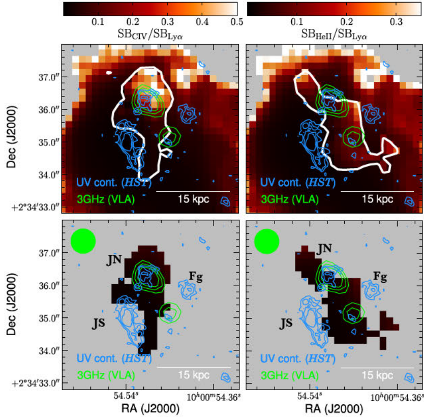
Figure 9. Upper panels: Spatial distributions of the C IV/Ly \alpha and He II/Ly \alpha SB ratios. The white contour delimits the region where C IV or He II is detected at a SNR > 3. The blue contours show the rest-frame UV continuum from the HST /F160W imaging and the lime contours display the VLA 3 GHz radio continuum emission (Smolčić et al. 2017b). Contour levels are the same as in Fig. 2. The pixel values outside the white contours are 1\sigma upper limits to the C IV/Ly \alpha and He II/Ly \alpha SB ratios (see the text for details). Lower panels: Spatial distribution of the 1\sigma uncertainties of the C IV/Ly \alpha and He II/Ly \alpha SB ratios. The VLA beam shape is shown in the upper-left corners. The regions with the highest C IV/Ly \alpha and He II/Ly \alpha ratios are located in the vicinity of J1000+0234–North (JN): a massive SMG, with signatures of AGN activity, that has a UV and 3 GHz radio counterpart. The lowest C IV/Ly \alpha and He II/Ly \alpha SB ratios, with a 1\sigma upper limit of \approx 0.003 , are located at the locus of J1000+0234–South (JS): a low-mass SFG that is bright in the UV and no signatures of AGN activity.
