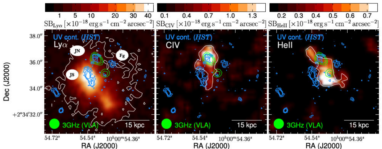
Figure 2. Optimally extracted SB maps of \text{Ly } \alpha (left-hand panel), CIV (middle panel), and He II (right-hand panel) emission of J1000+0234. In the case of CIV and He II, we apply a spatial boxcar smoothing ( 2 \times 2 pixels) to the cube before producing the SB maps (using the option -boxsm in CUBEX). The thin white contours indicate the \text{SNR} = 3 isophote. The blue contours show the rest-frame UV continuum from the HST /F160W imaging and the lime contours display the VLA 3 GHz radio continuum emission at 0.75 arcsec resolution (Smolčić et al. 2017b). The former are plotted at 3, 5, and 8 times the rms noise level, while the latter are drawn at 3, 4, and 5 times the rms noise level. The VLA beam shape is shown at the bottom-left corner. There are three prominent UV sources within the extended \text{Ly } \alpha blob: a southern component associated with a low-mass SFG (J1000+0234–South; JS), a northern UV emitting source linked to a massive SMG (J1000+0234–North; JN) with a 3 GHz radio counterpart, and a foreground ‘Fg’ galaxy at z = 1.41 (Capak et al. 2008; Gómez-Guijarro et al. 2018). While the brightest \text{Ly } \alpha region matches the locus of the low-mass SFG, the brightest CIV region is coincident with the SMG position. He II emission is maximal at \approx 0.6 arcsec to the south-east of a compact 3 GHz radio source that has a faint UV counterpart.
