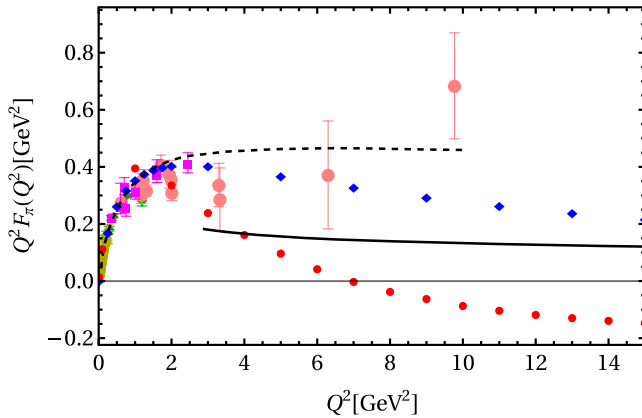
FIG. 4. Charged pion electromagnetic form factor. Experimental points are shown by dark yellow triangles [102], green diamonds [103], pink circles [104–106], and magenta squares [107–110]. Red solid circles and blue diamonds are calculated using the ADFM quark-propagator Ansatz and the MMF quark-propagator Ansatz , respectively. In the case of the MMF quark propagator, three different methods of calculation (detailed in the text) yielded the same results. The black dashed line represents the result of Mello et al. [19]. The black solid line corresponds to the perturbative QCD result (27) with asymptotic PDA.
