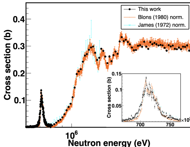
FIG. 15. Cross section of the ^{230}\text{Th}(n, f) reaction (black circle), estimated using the ^{235}\text{U}(n, f) reaction as reference, plotted along with the data of Blons et al. (orange points) and James et al. (cyan cross) normalized to the current data. Only the statistical uncertainties are shown in the figure.
