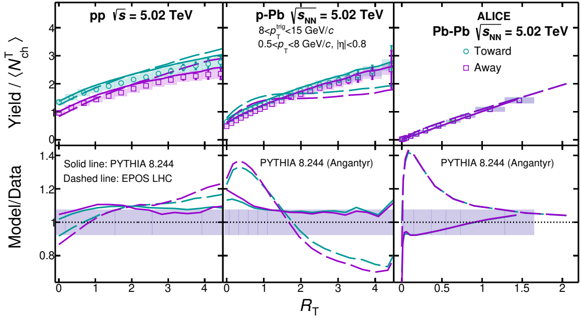
Figure 9. Top: integrated yield of charged particles in pp (left), p-Pb (middle), and Pb-Pb (right) collisions at \sqrt{s_{NN}} = 5.02 TeV as a function of R_T for toward and away regions compared with predictions from EPOS LHC and PYTHIA 8. Bottom: ratio of model predictions to data. The band around unity in the ratio depicts the experimental uncertainties.
