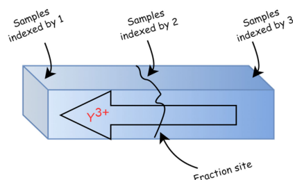
Scheme 1. Schematic representation of Y-TZP bar samples prepared using CAD/CAM technology in this work. The content of Y^{3+} is increasing from the right (i.e., 3Y-TZP) to the left (i.e., 5Y-TZP). These bar samples are considered multilayers due to varying Y^{3+} amounts, which lead to changes in transparency and the materials' mechanical, structural, and morphological properties.
