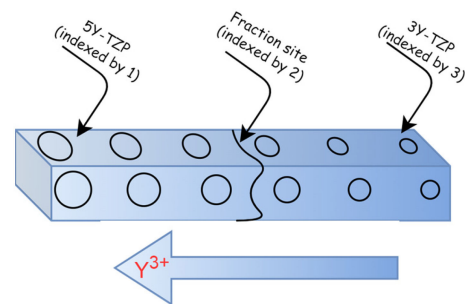
Scheme 3. Schematic representation of bar samples used in this work. The grain sizes are arbitrarily chosen for illustration purposes. The scheme depicts a trend of increasing grain size alongside Y^{3+} content, which correlates with the trend presented in Figure 4. According to manufacturers, the size of the grains is governed by the Y^{3+} content; however, the exact layer composition is not designated.
