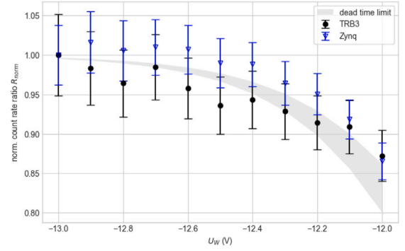
Fig. 3. Test of the NDET readout rate capability. The normalized rate is shown as a function of the Wehnelt voltage (see text for explanations). The ratios are shown for both readout methods, Zynq and TRB3 board. The grey band indicates the expected ratio for signals with a Time-over-Threshold between 45 ns and 65 ns as observed during the experiment.
