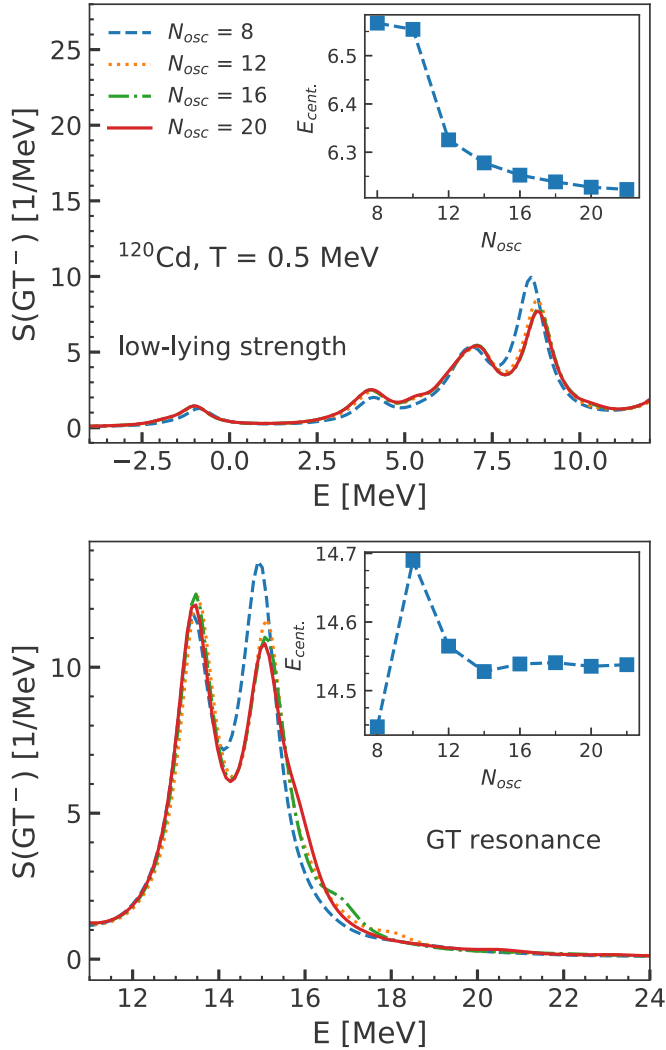
FIG. 4. The GT - strength function with respect to the number of oscillator shells N_{\text{osc}} in ^{120}\text{Cd} at T = 0.5 MeV. The number of Gauss-Hermite integration mesh points is set to N_{\text{gh}} = 24 and number of pairing interaction terms is N_{\text{pp}} = 8 . In the upper panel the low-lying GT strength is shown for different N_{\text{osc}} together with its centroid energy E_{\text{cent.}} in the inset. In the lower panel the same is displayed for the GT resonance region.
