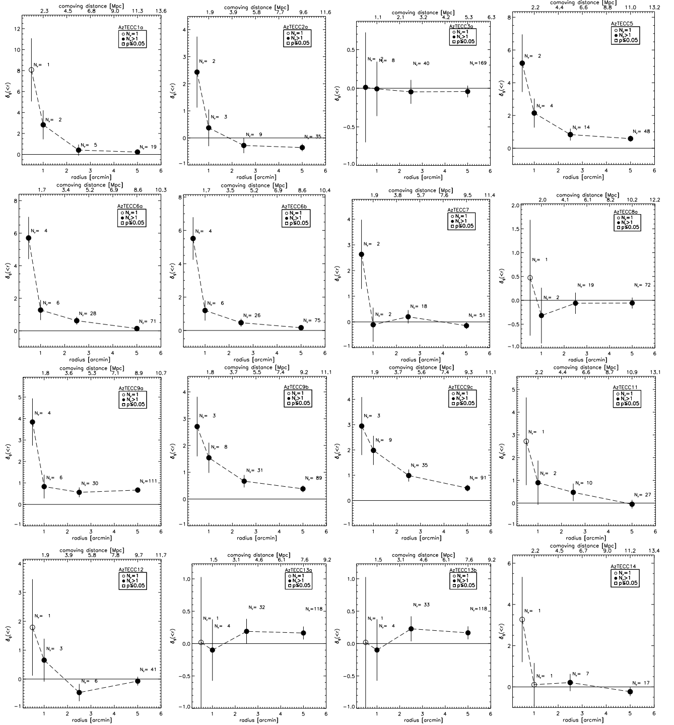
Fig. A.1. Overdensity parameter \delta_g vs. radius r measured from the central SMG. Open dots represent when the only source measured within that radius is the target SMG, and black dots represent when at least one more source than the central SMG is observed. Error bars represent Poissonian errors. The dot is enclosed in a square when Poisson probability is p \leq 0.05 . The name of each SMG is indicated in the legend and the number of sources found within a radius r is indicated next to each point. A horizontal line represents \delta_g = 0 .
