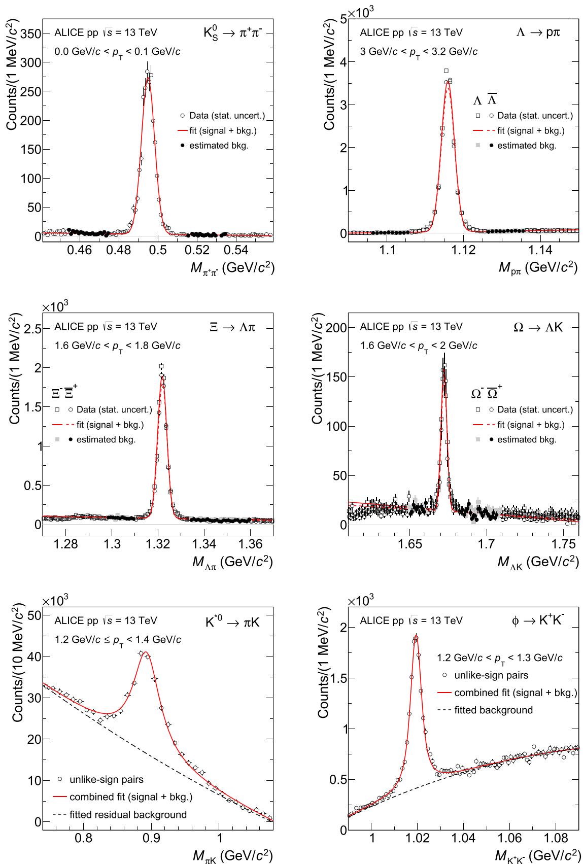
Fig. 4 Invariant mass distributions of K_S^0 , \Lambda and \bar{\Lambda} , \Xi^- and \bar{\Xi}^+ , and \Omega^- and \bar{\Omega}^+ , K^{*0} and \bar{K}^{*0} and \phi . See the text for details
