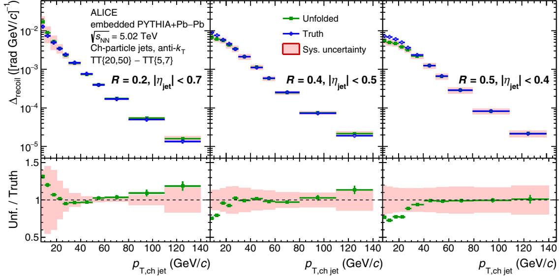
FIG. 10. Closure test of \Delta_{recoil}(p_{T, jet}) analysis for central Pb-Pb collisions.
