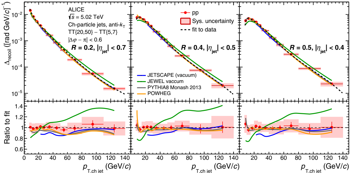
FIG. 11. (upper panels) corrected \Delta_{recoil}(p_{T, ch jet}) distributions measured for R = 0.2 (left), 0.4 (middle), and 0.5 (right) in pp collisions at \sqrt{s} = 5.02 TeV, compared with calculations from JETSCAPE [110], JEWEL [115,116], PYTHIA8 [99,100], and POWHEG [102–105]. (lower panels) Ratio of the data and calculations to a functional fit of the measured \Delta_{recoil}(p_{T, ch jet}) distributions.
