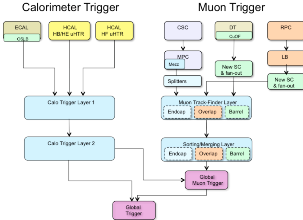
Figure 3.11: Schematic layout of L1 trigger system of the CMS experiment [69].
