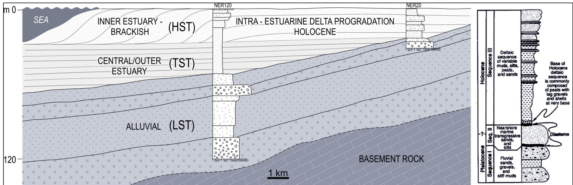
Figure 6.14. Schematic longitudinal profile through Neretva river delta sediments indicating depositional environments during Pleistocene and Holocene. The interpretation is based on differences in grain size distribution in the cores NER120 and NER20.
