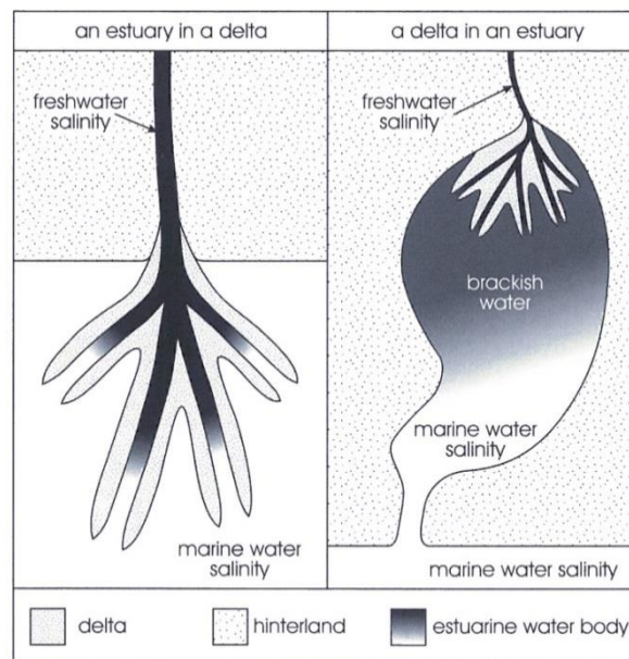
Figure 2.7. Idealised diagram showing the dual concept of an estuary within a large delta and a delta within a large estuary (or an intra-estuarine delta). Legend: freshwater = black; brackish water = gray; marine water = white (Kennish, 2016).
