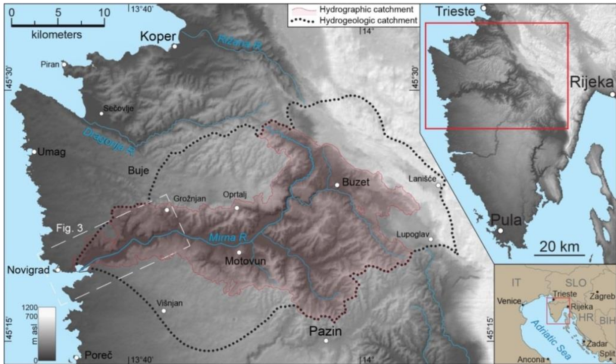
Figure 3.1. Location of the study area (Mirna River and its drainage area). The Digital Elevation Model (DEM) obtained from NASA-SRTM data. The boundary of the hydrogeological catchment is assumed (according to SANTIN, 2013) (Felja et al., 2015).
