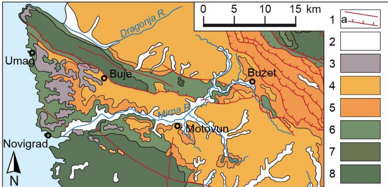
Figure 3.2. A geological map of Istria (modified after the Geological Map of Croatia 1:300000, Croatian Geological Survey, 2009); 1. Fault, 1a. Thrust, 2. Quaternary deposits (mainly Holocene), 3. Terra rossa deposits (Holocene), 4. Flysch deposits (Eocene), 5. Liburnia deposits, Foraminiferal limestone and transitional deposits (Paleocene?, Eocene), 6. Rudist limestone (Cretaceous), 7. Dolomite and breccia (Cretaceous), 8 Limestone and dolomite (Cretaceous) (Felja et al., 2015).
