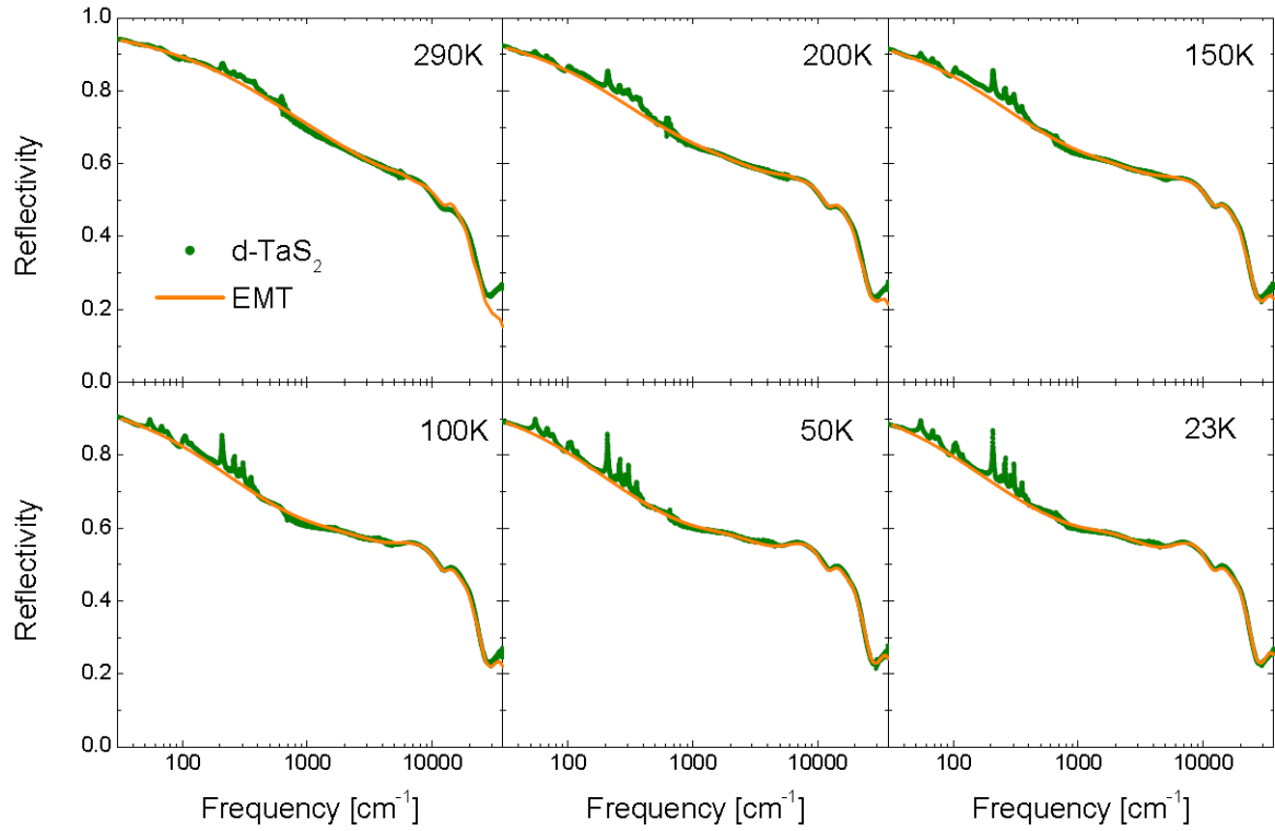
Figure 4.10. Three-component Bruggeman EMT fit (solid orange line) to the d\text{-TaS}_2 experimental reflectivity data (green circles).
