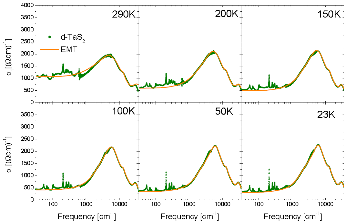
Figure 4.11. Three-component Bruggeman EMT fit (solid orange line) to the d\text{-TaS}_2 optical conductivity data (green circles).
