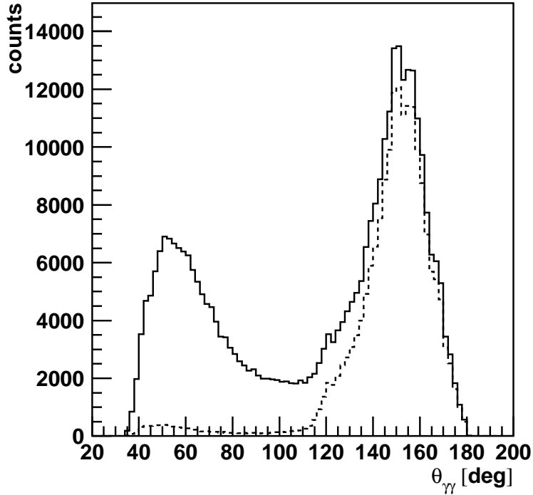
Figure 4.7: The photon opening angle distribution after tracking and clustering (solid line). The dashed line shows the distribution for photons with an energy deposition greater than 5 MeV.
