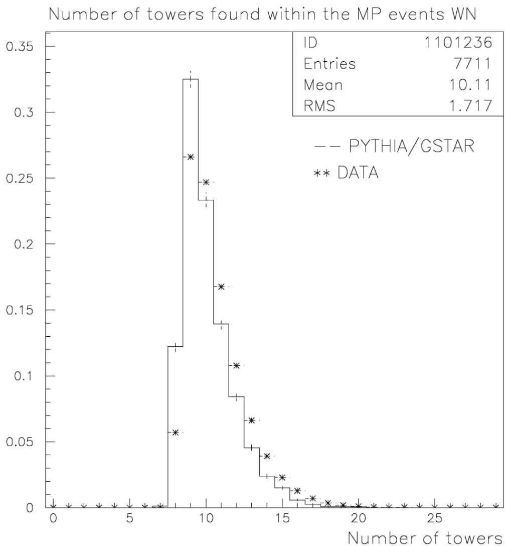
Figure 5.4: The number of towers in the multiphoton events in the WN calorimeter. The difference of the average value (shown on image for simulations) for data and simulations is about 5% and equals 10.66 for the data sample. The error bars are statistical.
