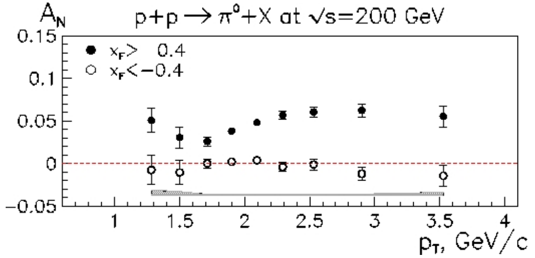
Figure 5.2: Calculated asymmetry for \pi^0 events in p_T bins for events with |x_F| > 0.4 [8].
