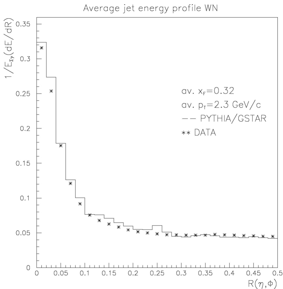
Figure 5.10: The 1/E_{mp.}(dE_{mp.}/dR) (jet profile) distribution for the energy bin corresponding to \langle x_F \rangle=0.32 in the WN module. The data and the simulation sample show very good agreement.
