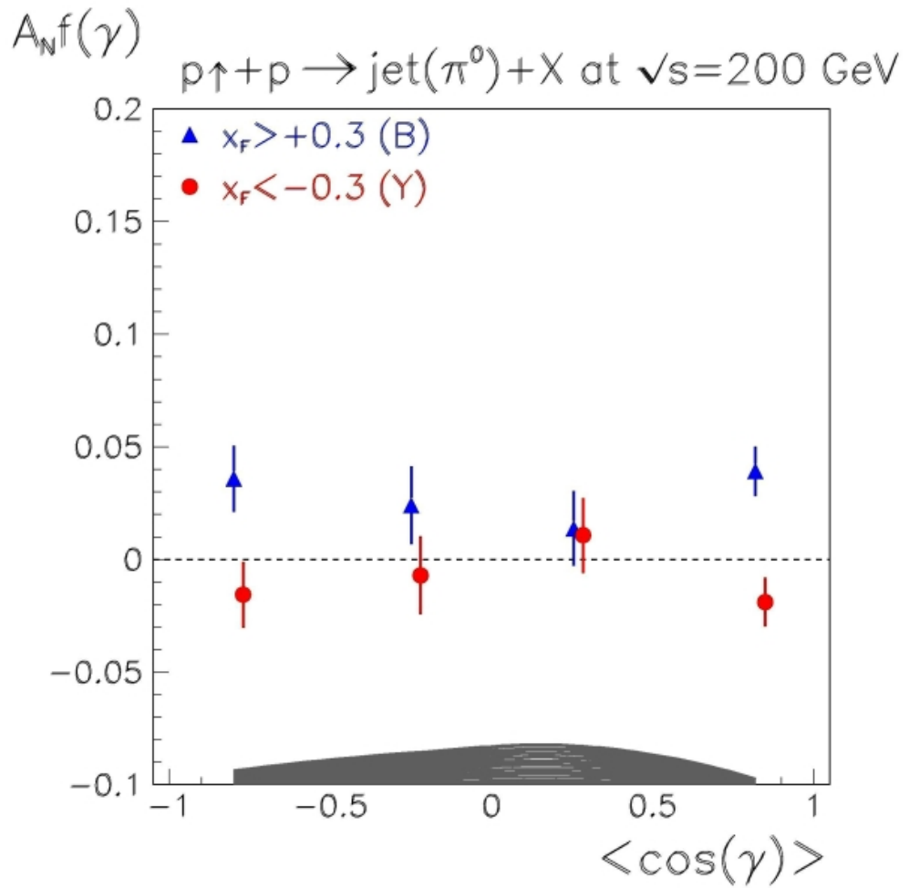
Figure 5.26: The calculated A_N as a function of \cos(\gamma) . The blue points correspond to the positive x_F values, the red points to the negative x_F values. The error bars on the points are statistical and the gray shaded area shows the systematical errors. The points for x_F > 0 and x_F < 0 have been slightly horizontally offset, so that all points are clearly visible.
